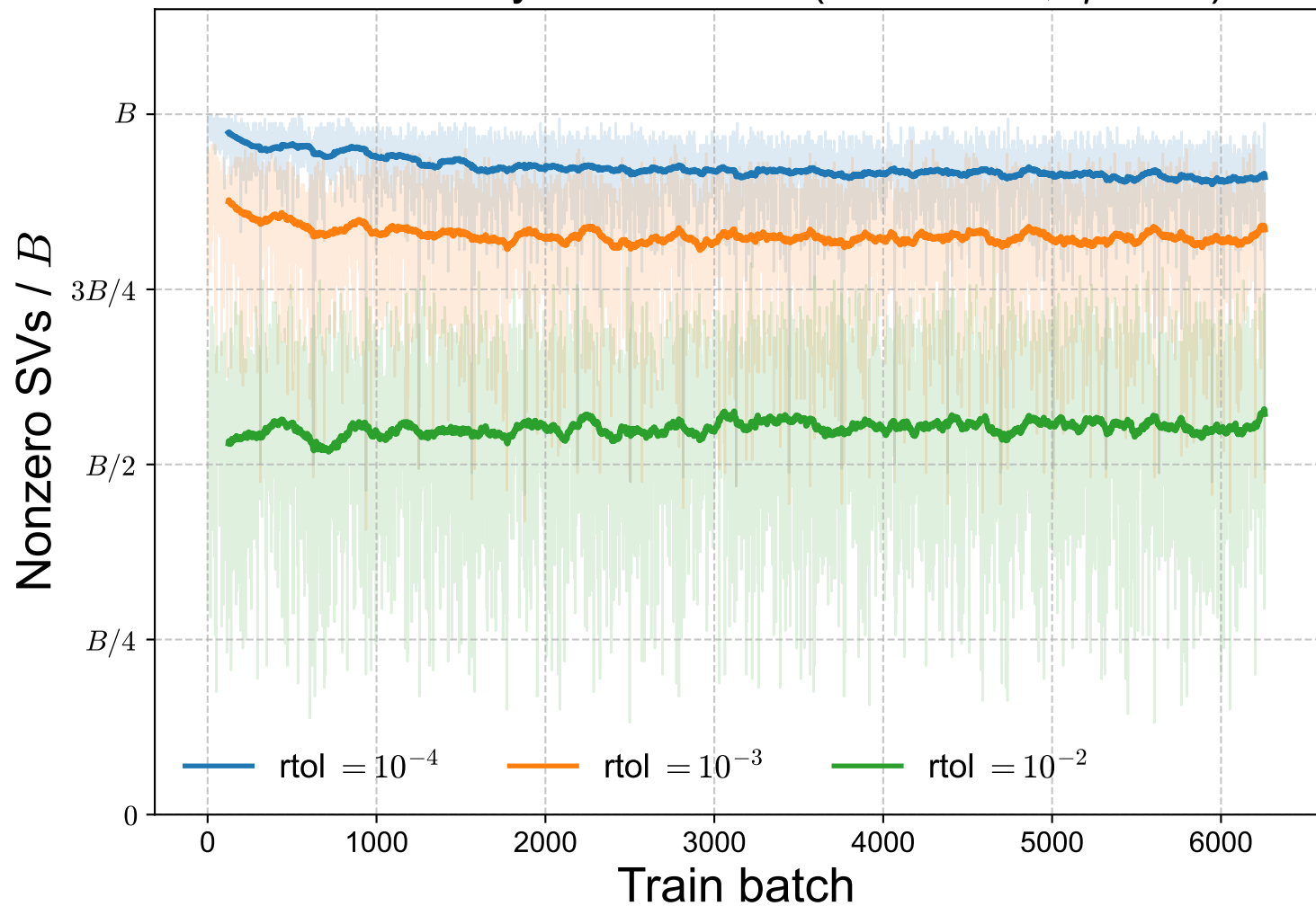
Random Polynomial: rank ( k = B = 32 , \eta = 0.5 )
