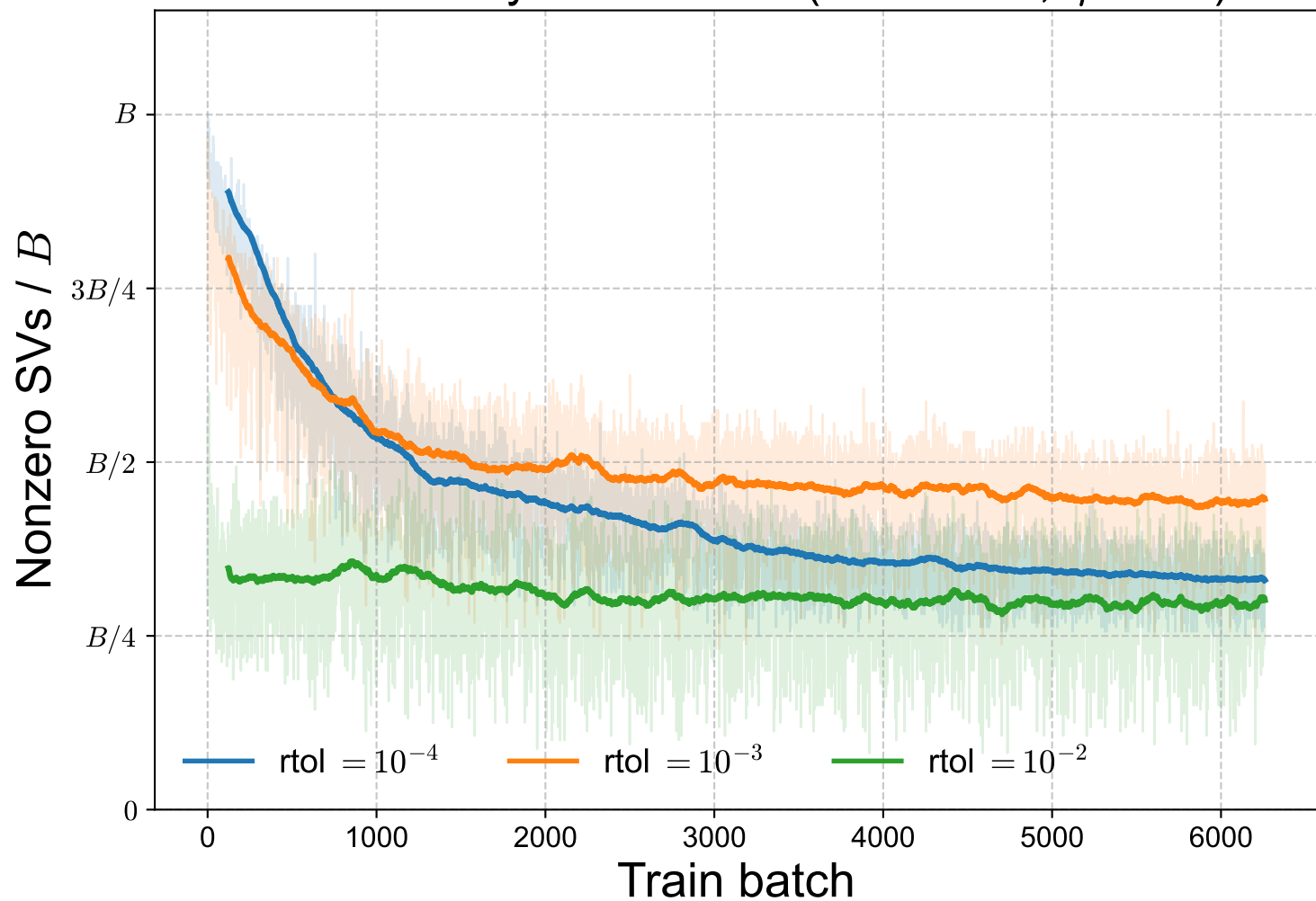
Random Polynomial: rank ( k = B = 32 , \eta = 10^0 )
