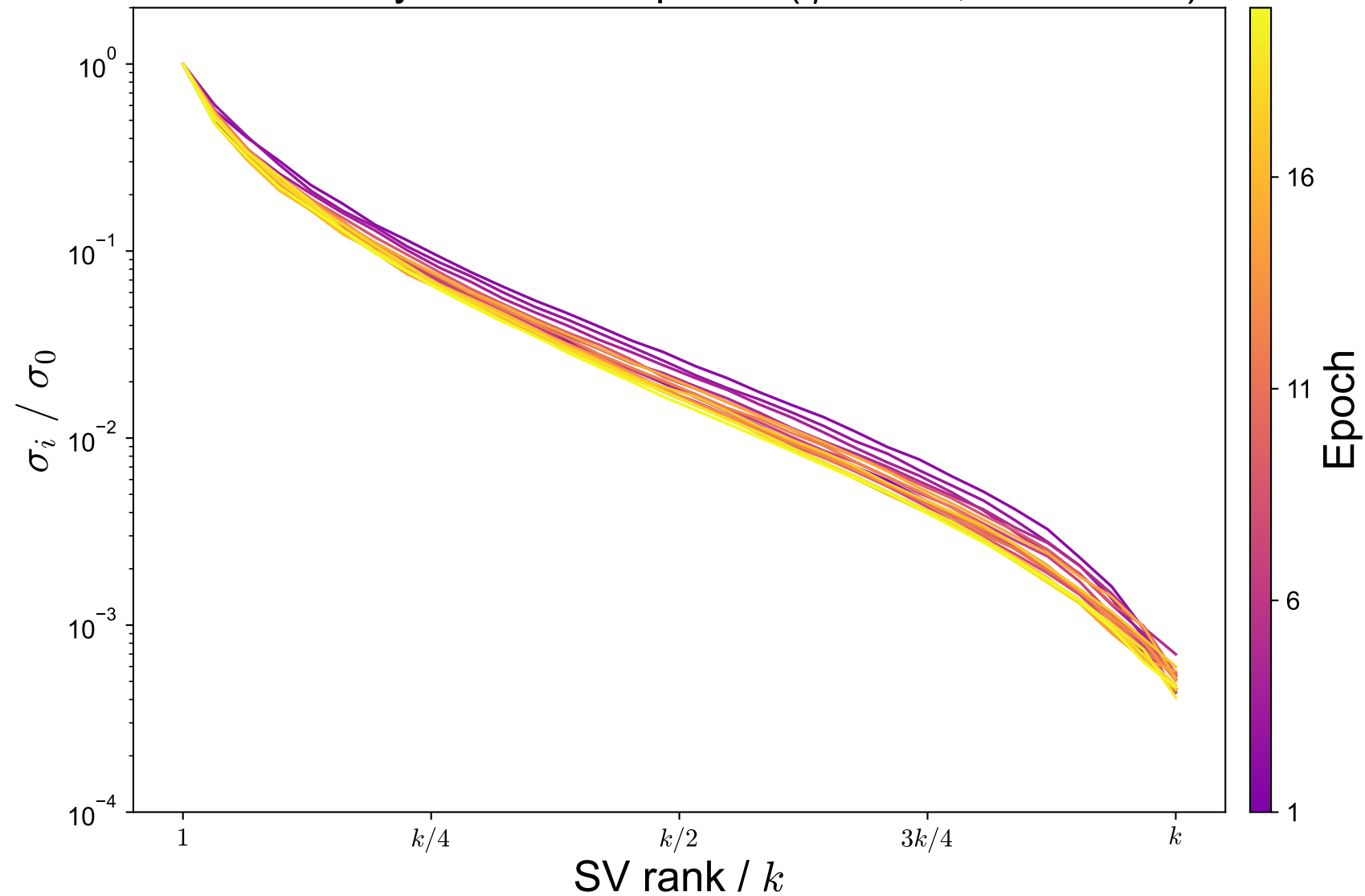
Random Polynomial: SV spectra ( \eta = 10^{-1} , \text{rtol} = 10^{-4} )
