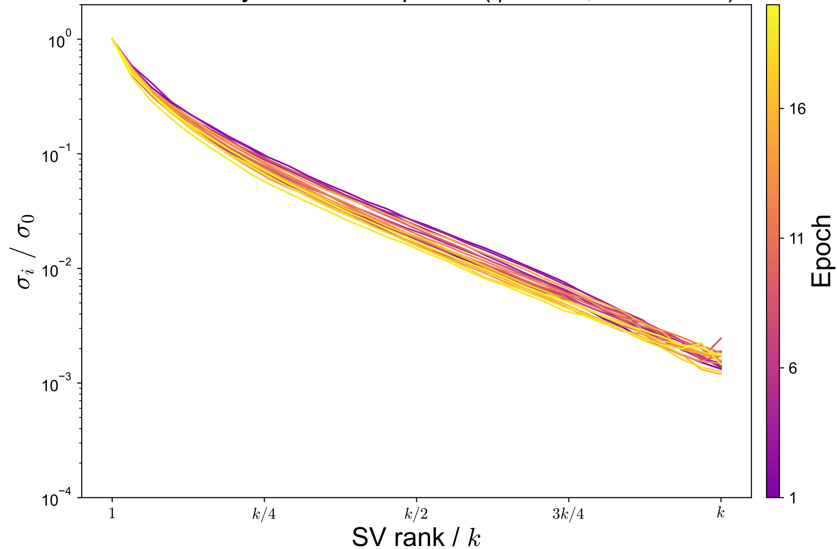
Random Polynomial: SV spectra ( \eta = 10^{-1} , \text{rtol} = 10^{-3} )
