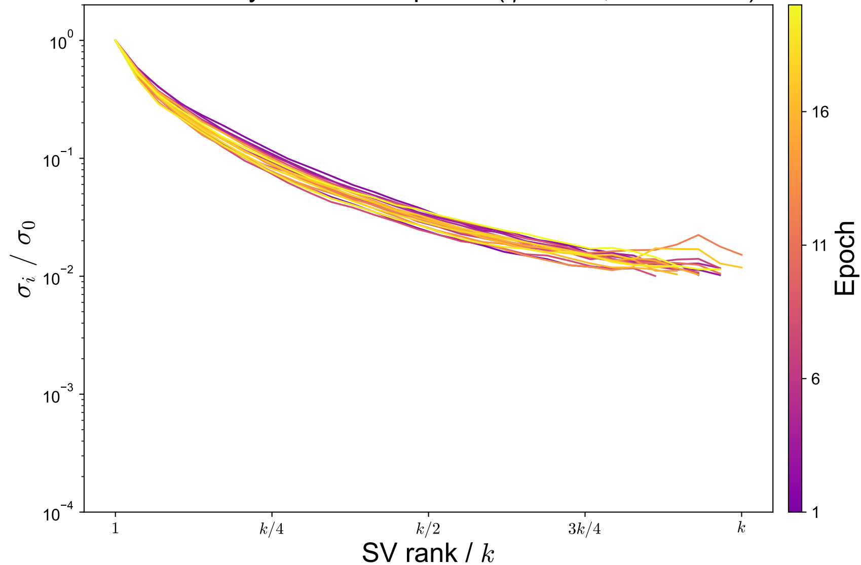
Random Polynomial: SV spectra ( \eta = 10^{-1} , \text{rtol} = 10^{-2} )
