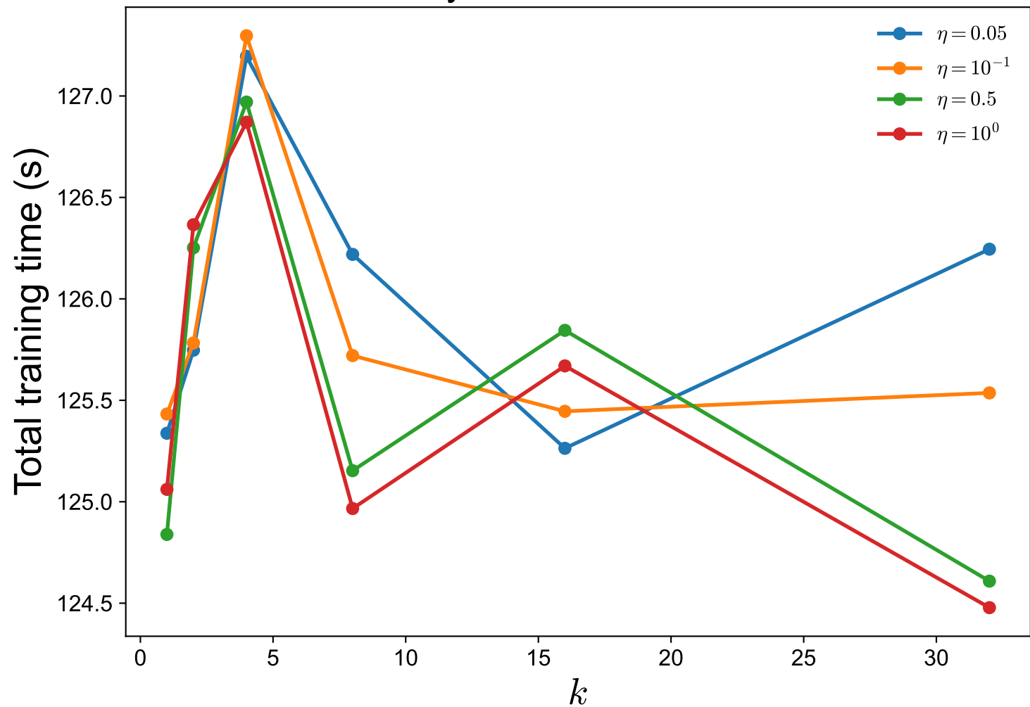
Random Polynomial: Sven wall time vs k
