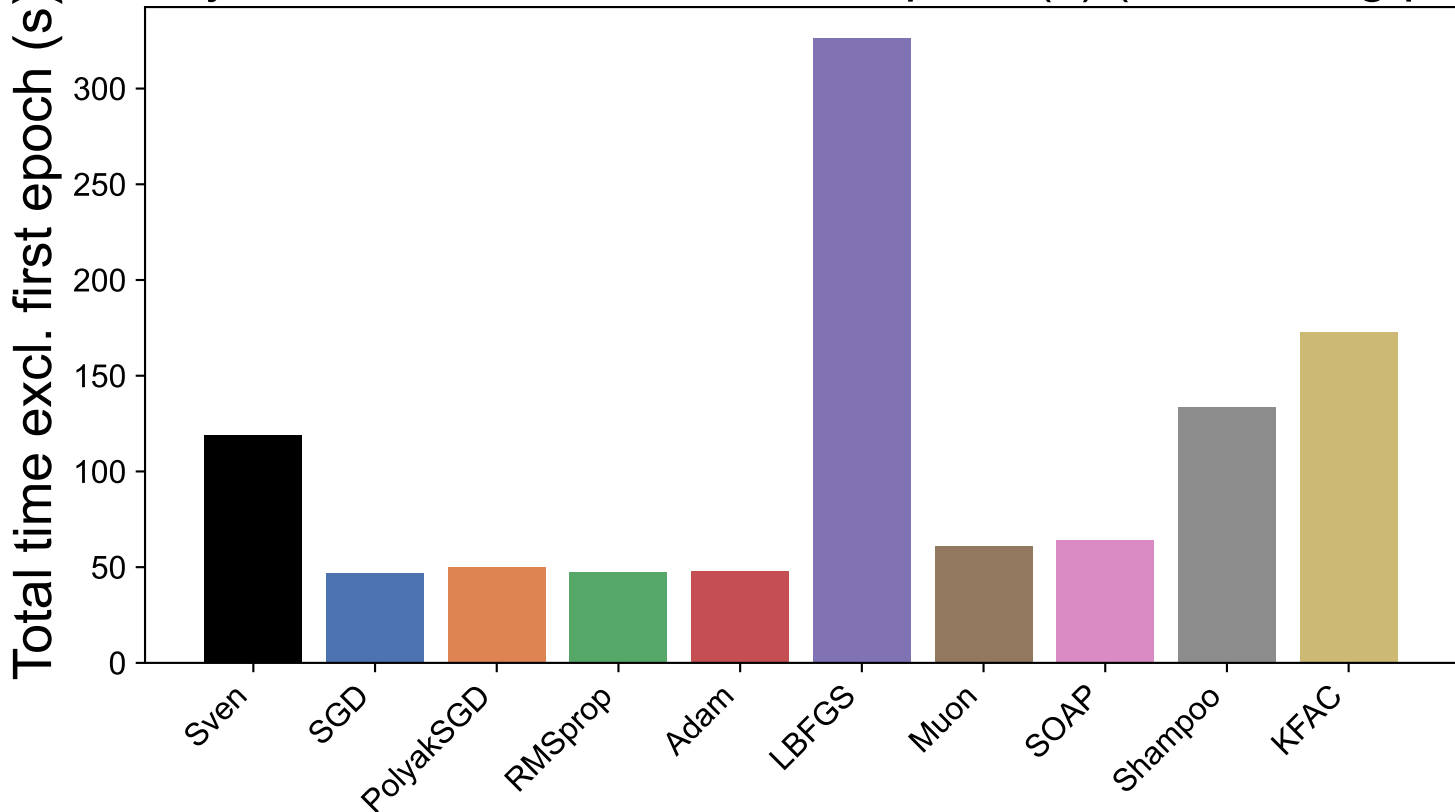
Random Polynomial: total time excl. first epoch (s) (best config per method)
