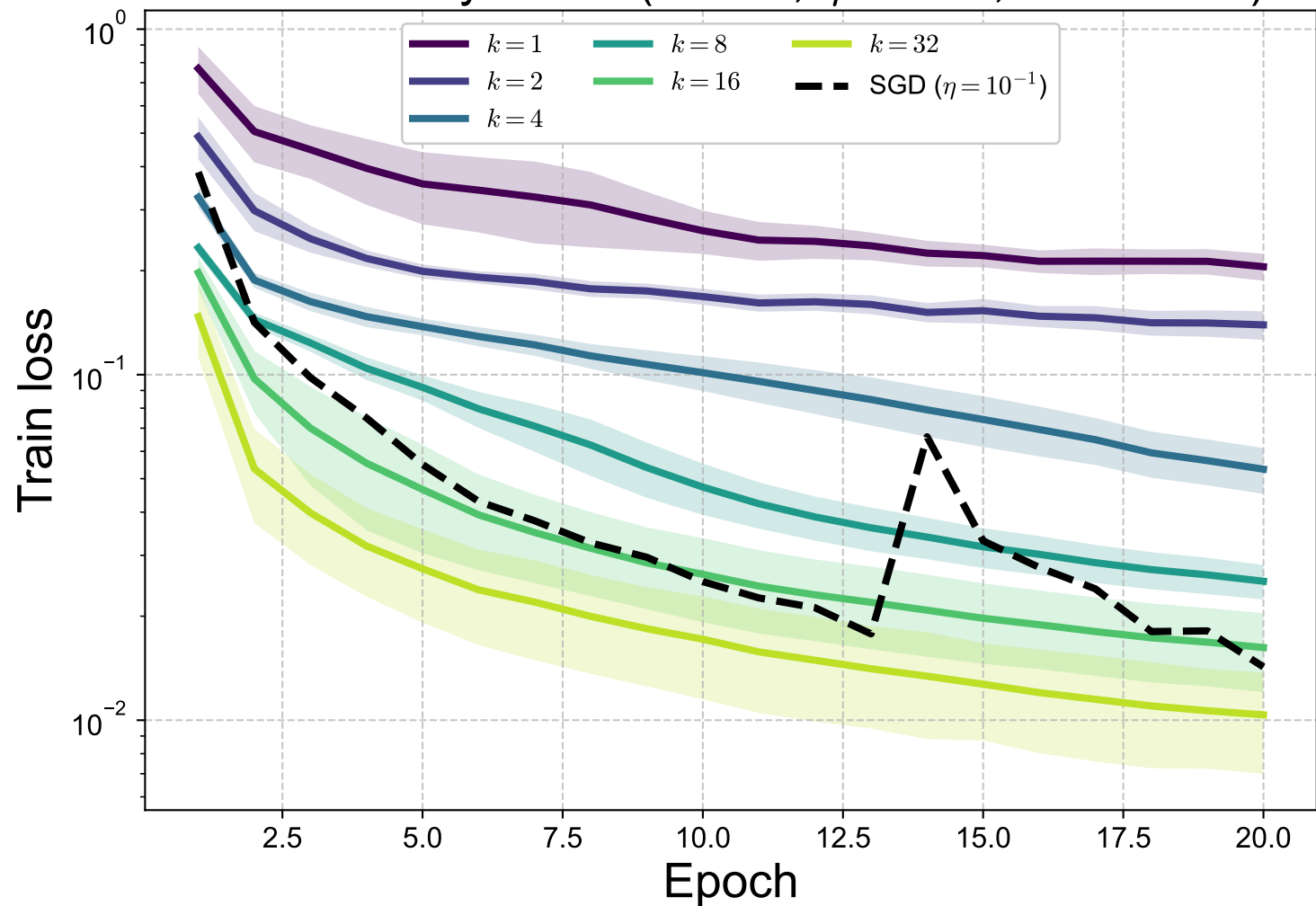
Random Polynomial ( B = 32 , \eta = 10^{-1} , \text{rtol} = 10^{-4} )
