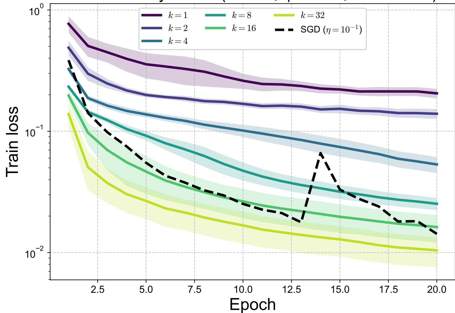
Random Polynomial ( B = 32 , \eta = 10^{-1} , \text{rtol} = 10^{-3} )
