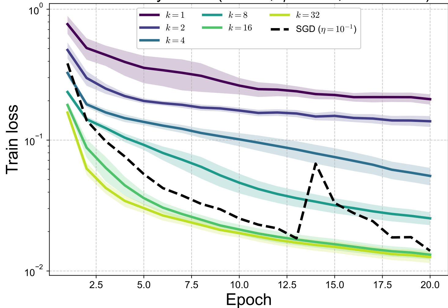
Random Polynomial ( B = 32 , \eta = 10^{-1} , \text{rtol} = 10^{-2} )
