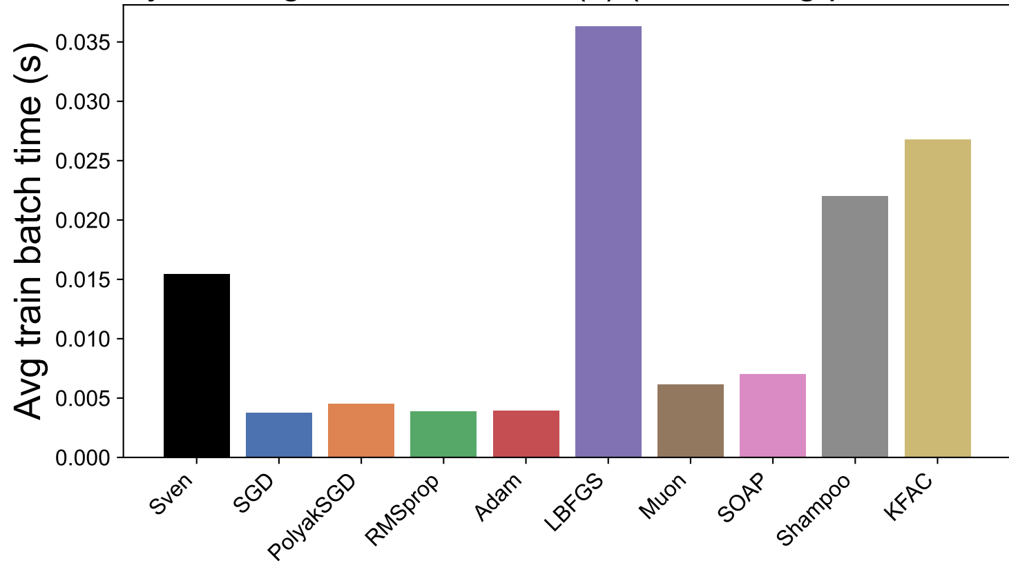
Toy 1D: avg train batch time (s) (best config per method)
