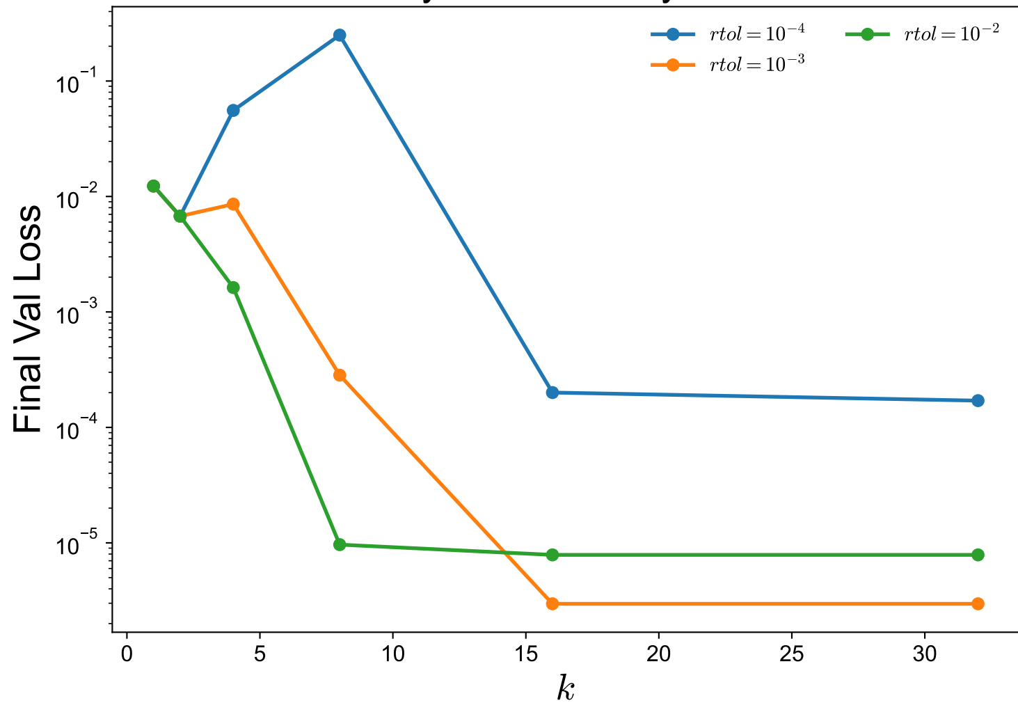
Toy 1D: sensitivity to k
