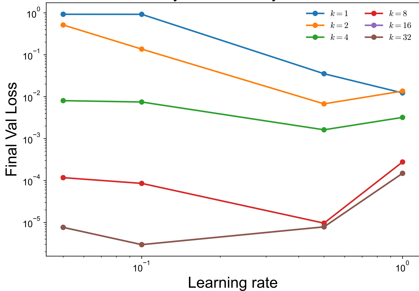
Toy 1D: sensitivity to \text{lr}
