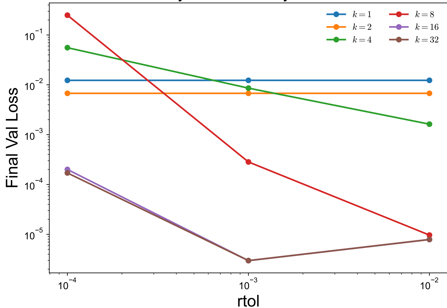
Toy 1D: sensitivity to rtol
