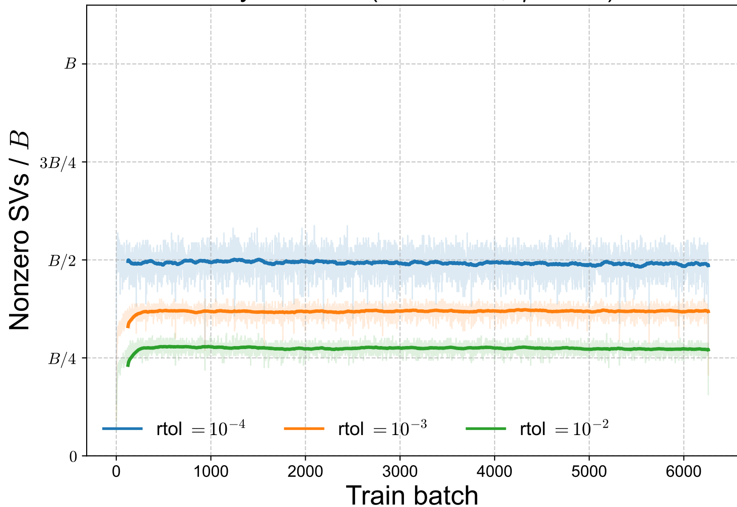
Toy 1D: rank ( k = B = 32 , \eta = 0.05 )
