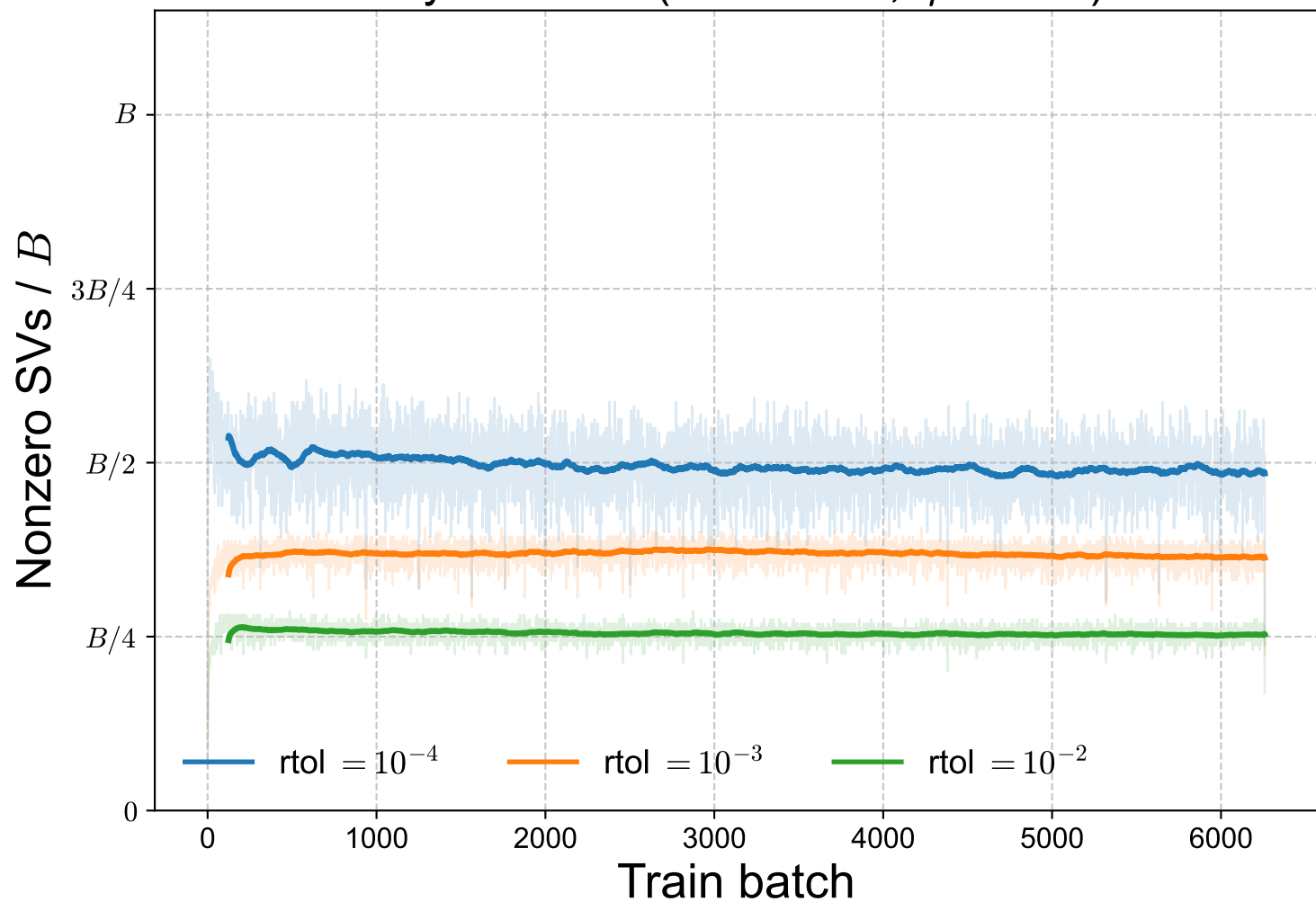
Toy 1D: rank ( k = B = 32 , \eta = 10^{-1} )
