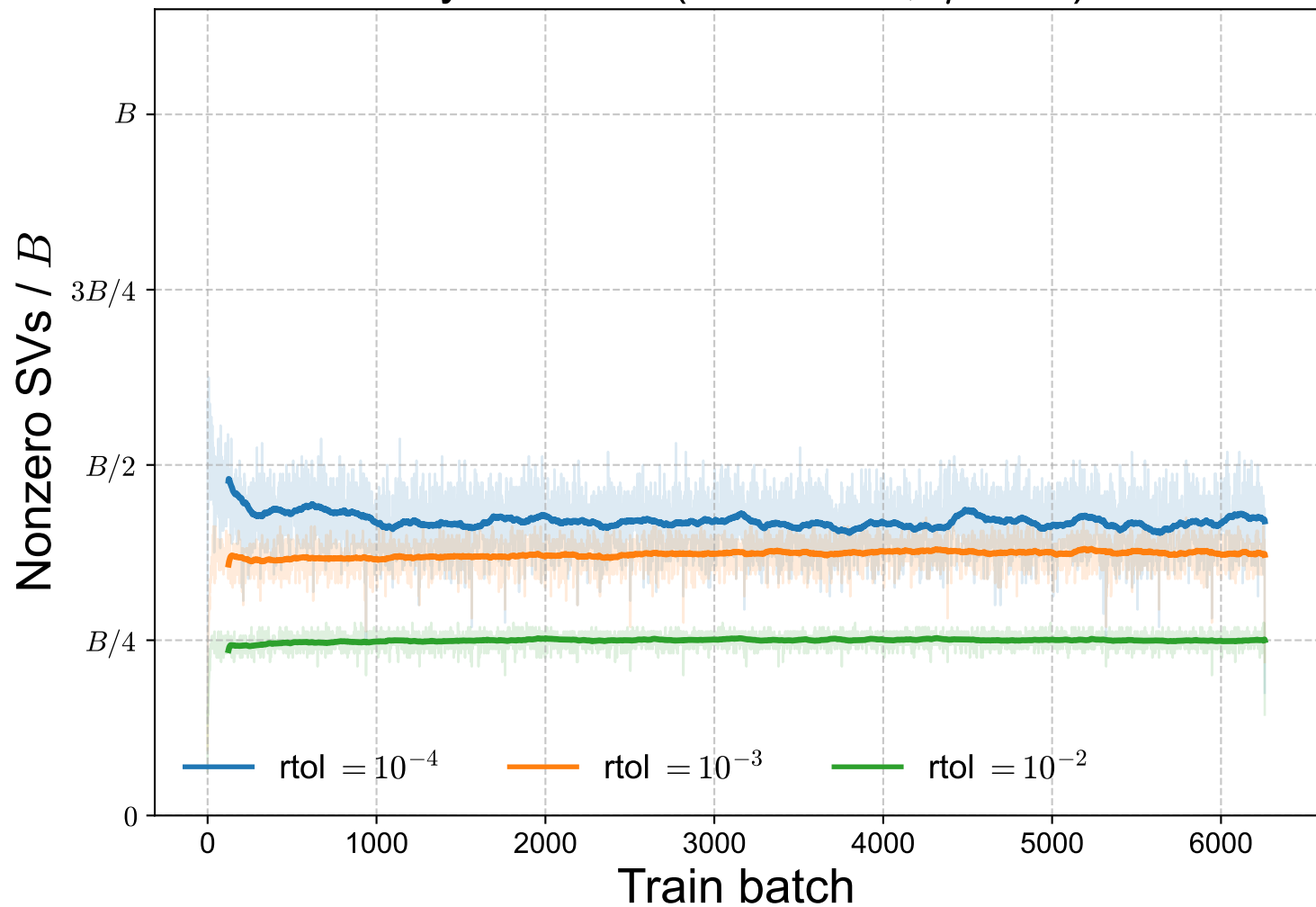
Toy 1D: rank ( k = B = 32 , \eta = 0.5 )
