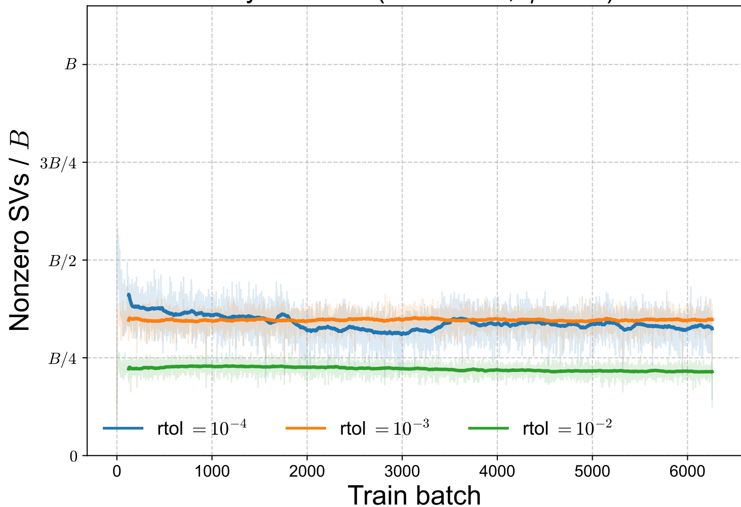
Toy 1D: rank ( k = B = 32 , \eta = 10^0 )
