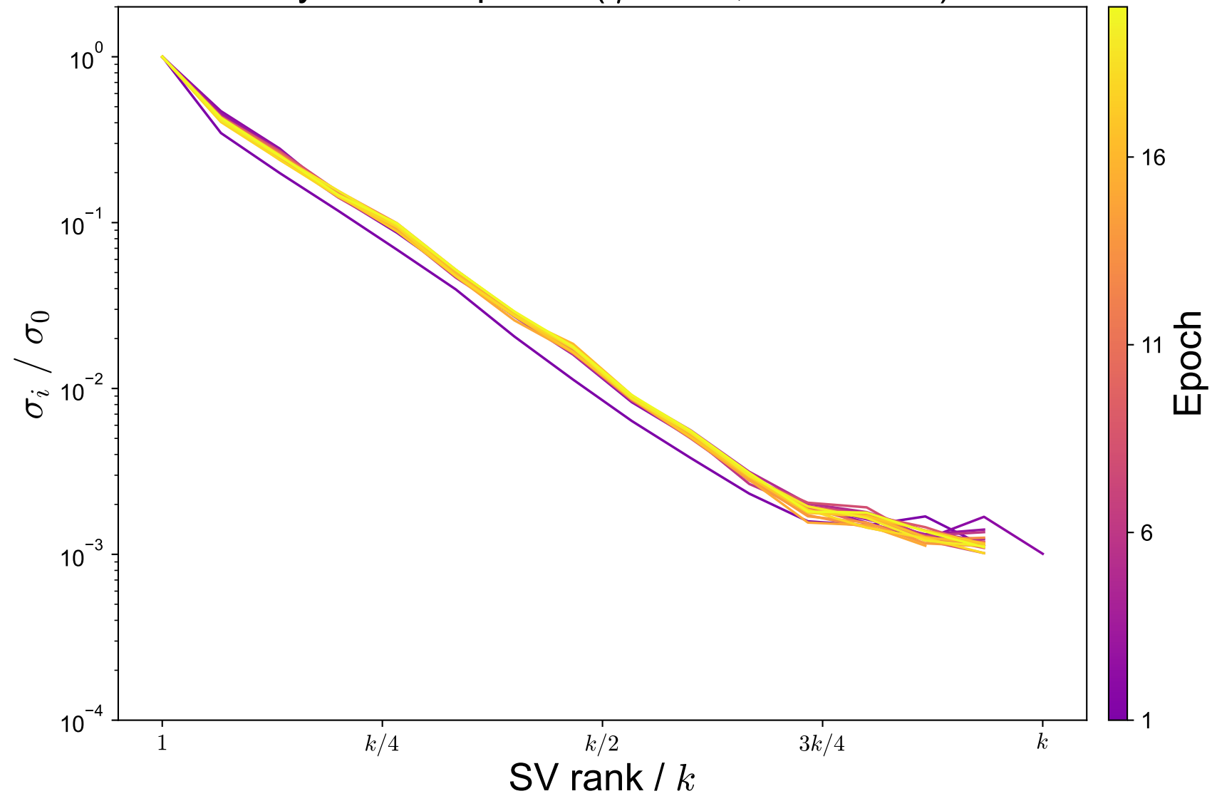
Toy 1D: SV spectra ( \eta = 0.05 , \text{rtol} = 10^{-3} )
