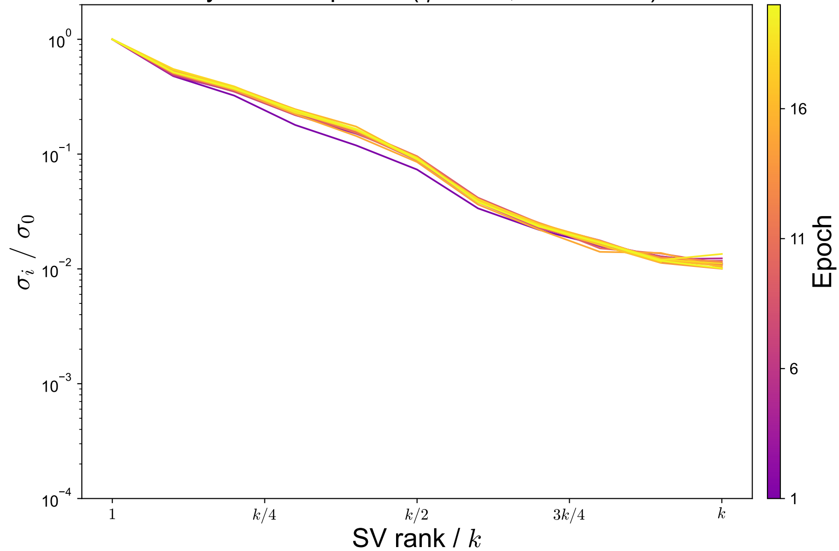
Toy 1D: SV spectra ( \eta = 0.05 , \text{rtol} = 10^{-2} )
