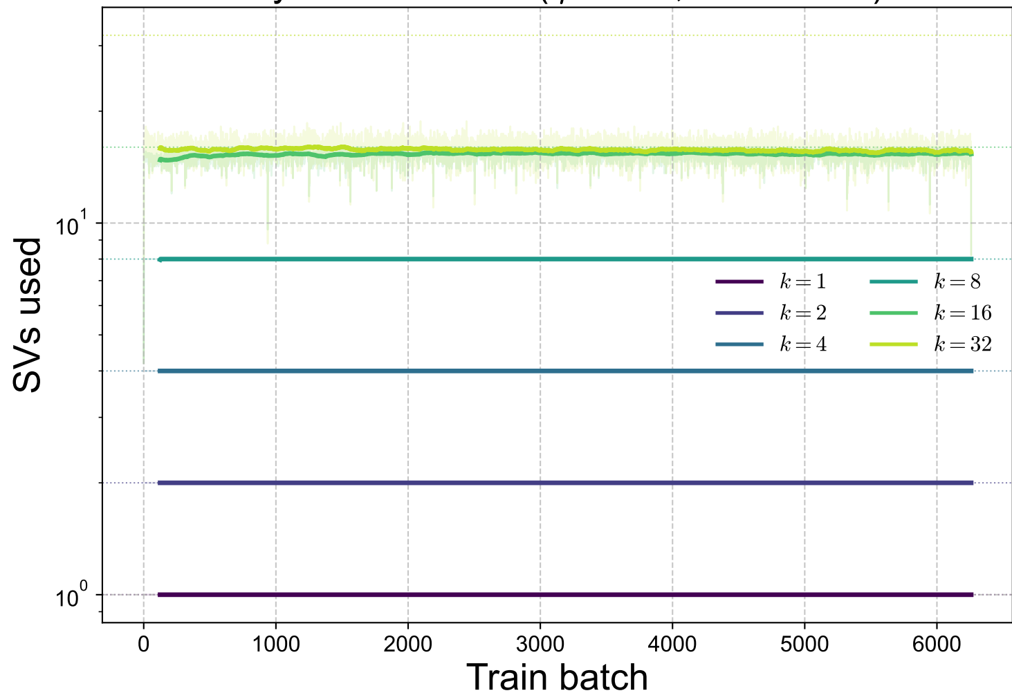
Toy 1D: SVs used ( \eta = 0.05 , \text{rtol} = 10^{-4} )
