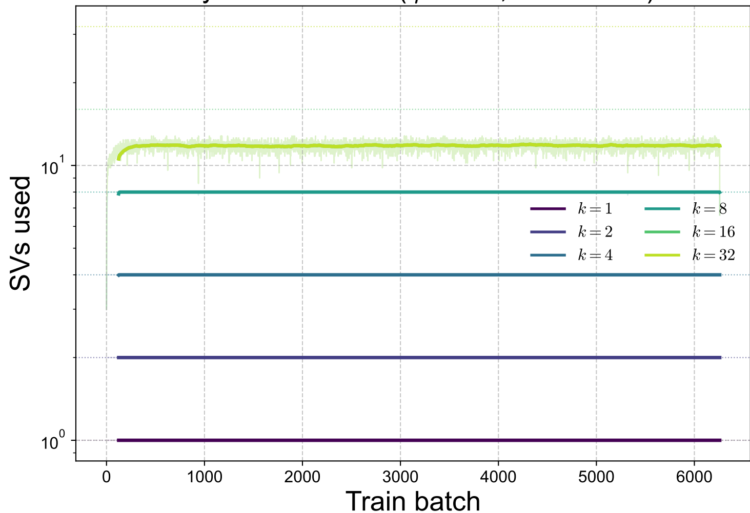
Toy 1D: SVs used ( \eta = 0.05 , \text{rtol} = 10^{-3} )
