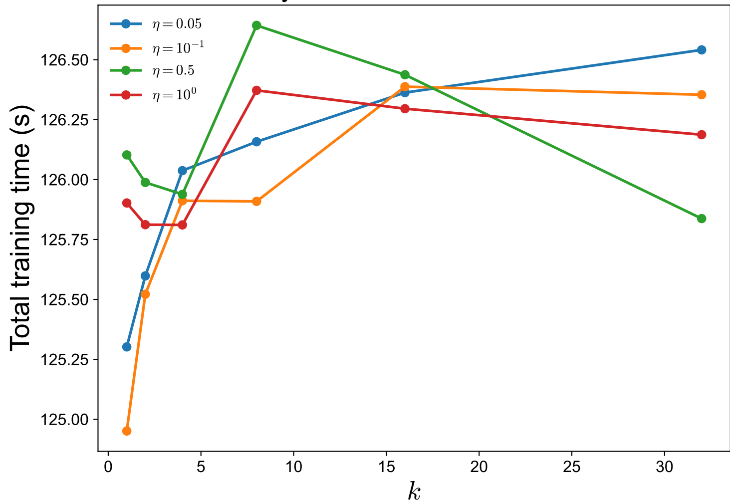
Toy 1D: Sven wall time vs k
