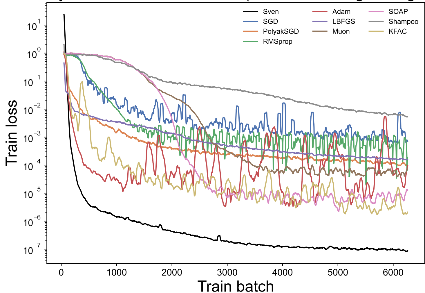
Toy 1D: batch-level train loss (50-batch moving average)
