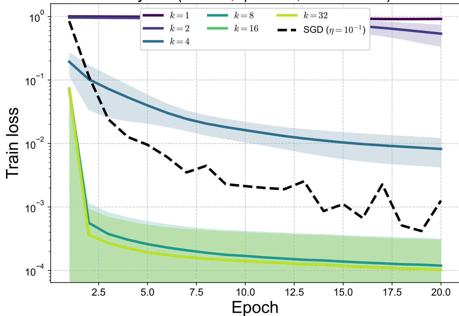
Toy 1D ( B = 32 , \eta = 0.05 , \text{rtol} = 10^{-2} )
