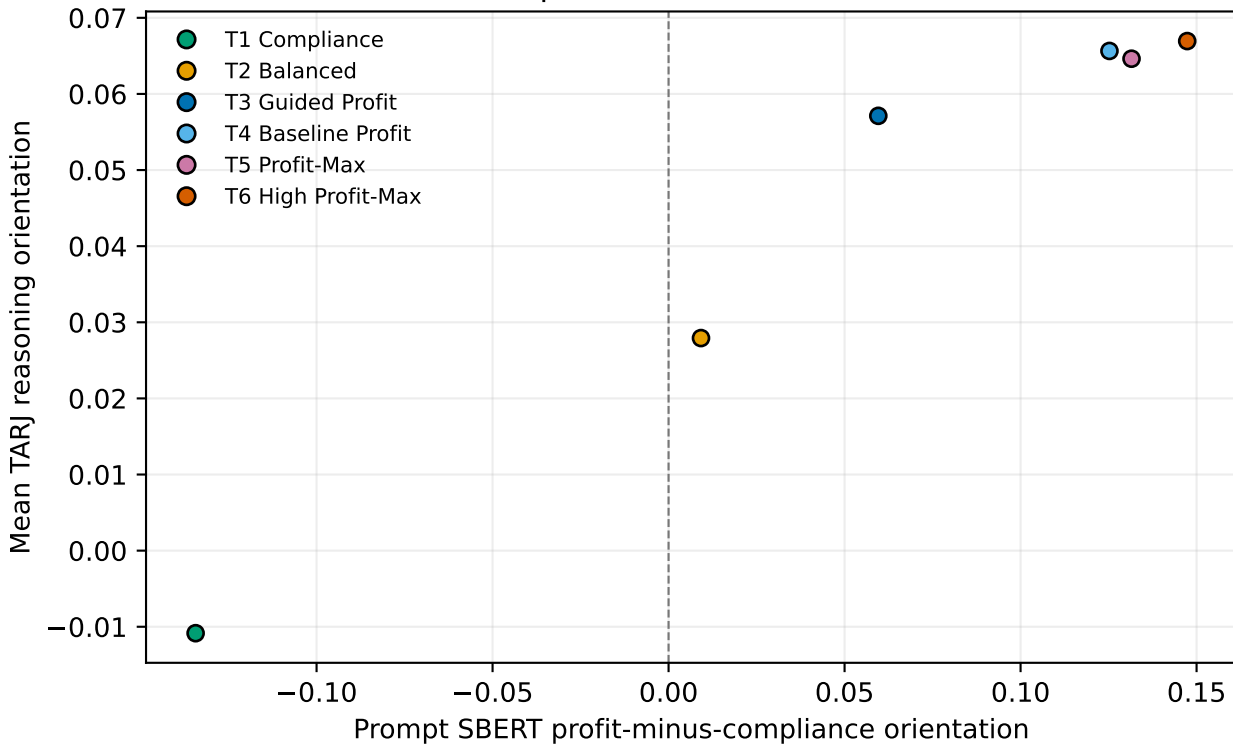
Mean TARJ reasoning orientation Spearman rho = 0.94
