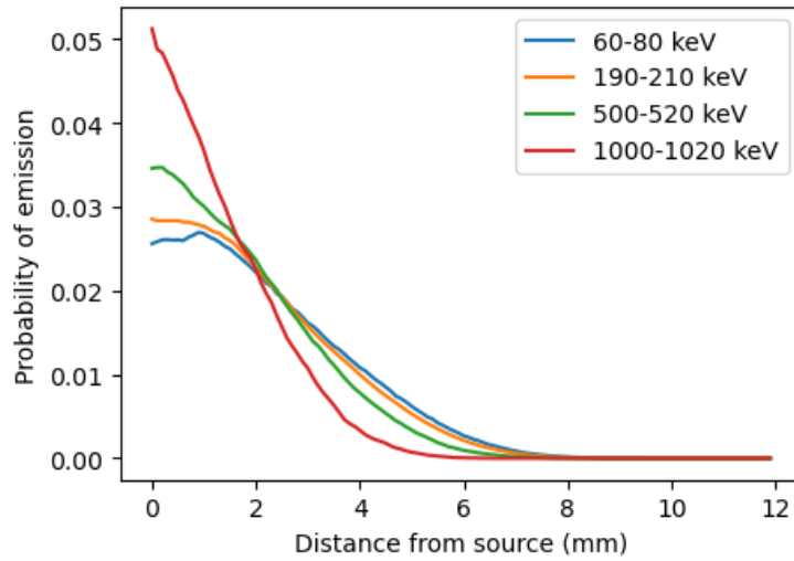
Figure 4.1: Plots showing probability of bremsstrahlung gamma emission versus the distance from ^{90}\text{Y} decay site. Data from Rault et al. [19]
