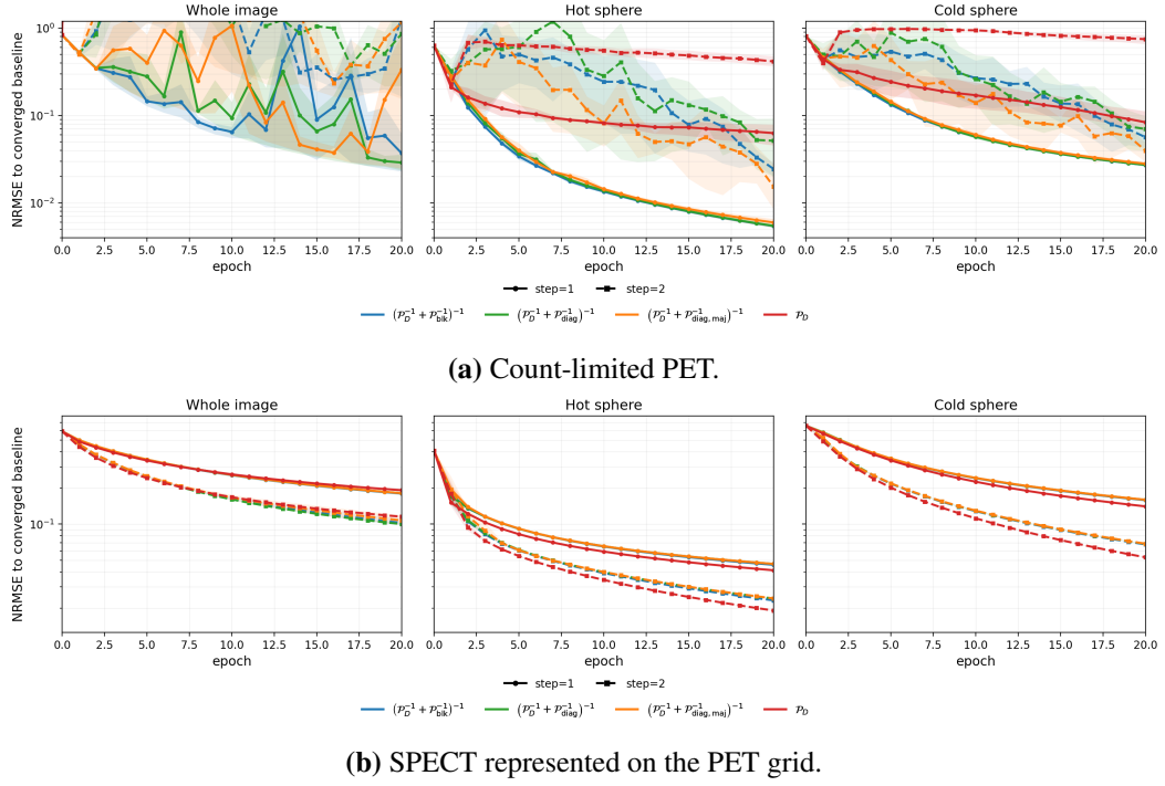
Figure 7.4: Sensitivity to the common initial step size for the displayed preconditioners. Solid curves use \zeta^{(0)} = 1 and dashed curves use \zeta^{(0)} = 2 . Lines and envelopes again show the five-run mean and pointwise minimum–maximum over 20 matched data passes.
