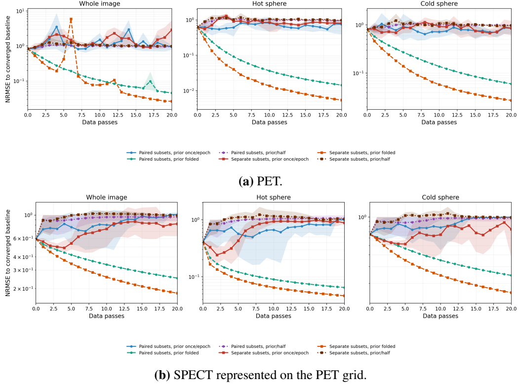
Figure 7.2: Convergence for the six combinations of subset organisation (paired, separate) and prior-application schedule (folded, sampled, once per epoch) using the MM local-diagonal curvature preconditioner. Lines show the mean per-run NRMSE over five stochastic realisations and shading shows the pointwise minimum–maximum over the first 20 matched data passes. In the legend, prior folded, prior/half, and prior once/epoch denote the folded, sampled, and once-per-epoch schedules; every schedule applies on average one complete prior contribution per matched data pass.
