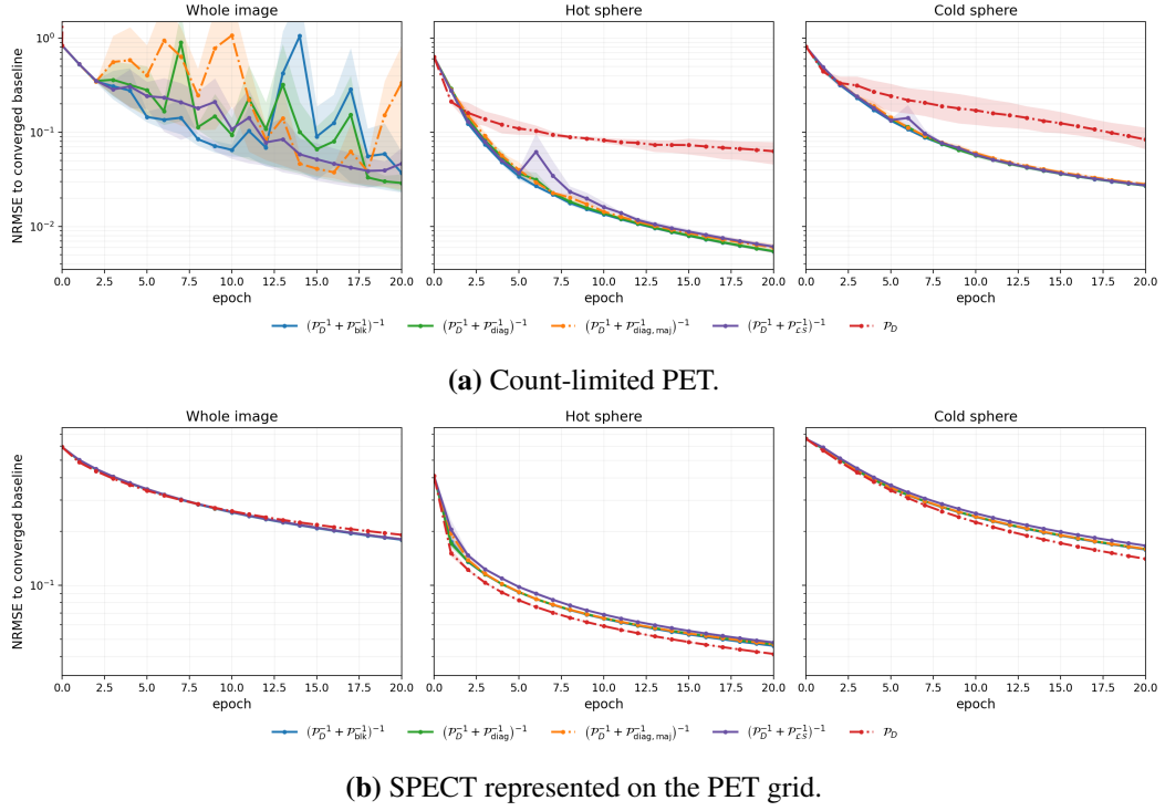
Figure 7.3: Convergence of data-only BSREM and the four prior-aware preconditioners in Table 7.1. All methods use the same objective and long-run reference within each modality. Lines show the mean per-run NRMSE over five stochastic realisations, and shading shows the pointwise minimum–maximum over the first 20 matched data passes.
