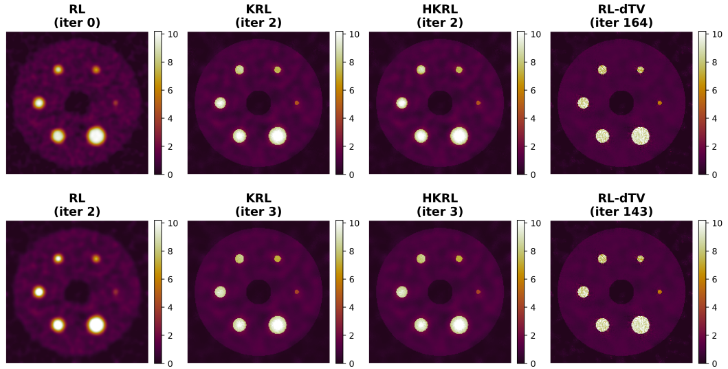
Figure 5.3: Figures showing central slice of reconstructions with best NRMSE. Top, initialised by the blurred PET image and bottom, initialised by a uniform image.
