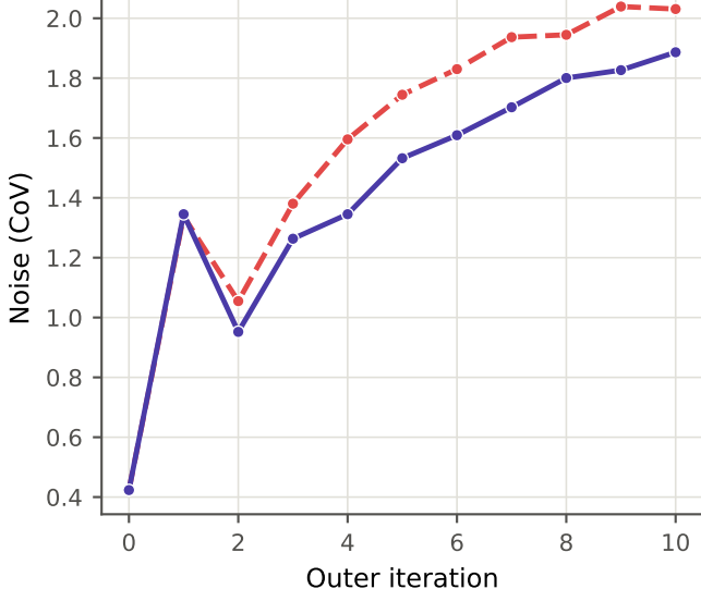
Damping stabilises the online scatter+residual update (NEMA (warm 8:1 background), updated scatter + residual, \beta = 0.0 )
