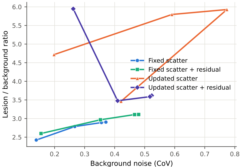
Patient (SIRT-3): lesion contrast vs noise ( \beta swept, brems blur on, PET-space lesions)
