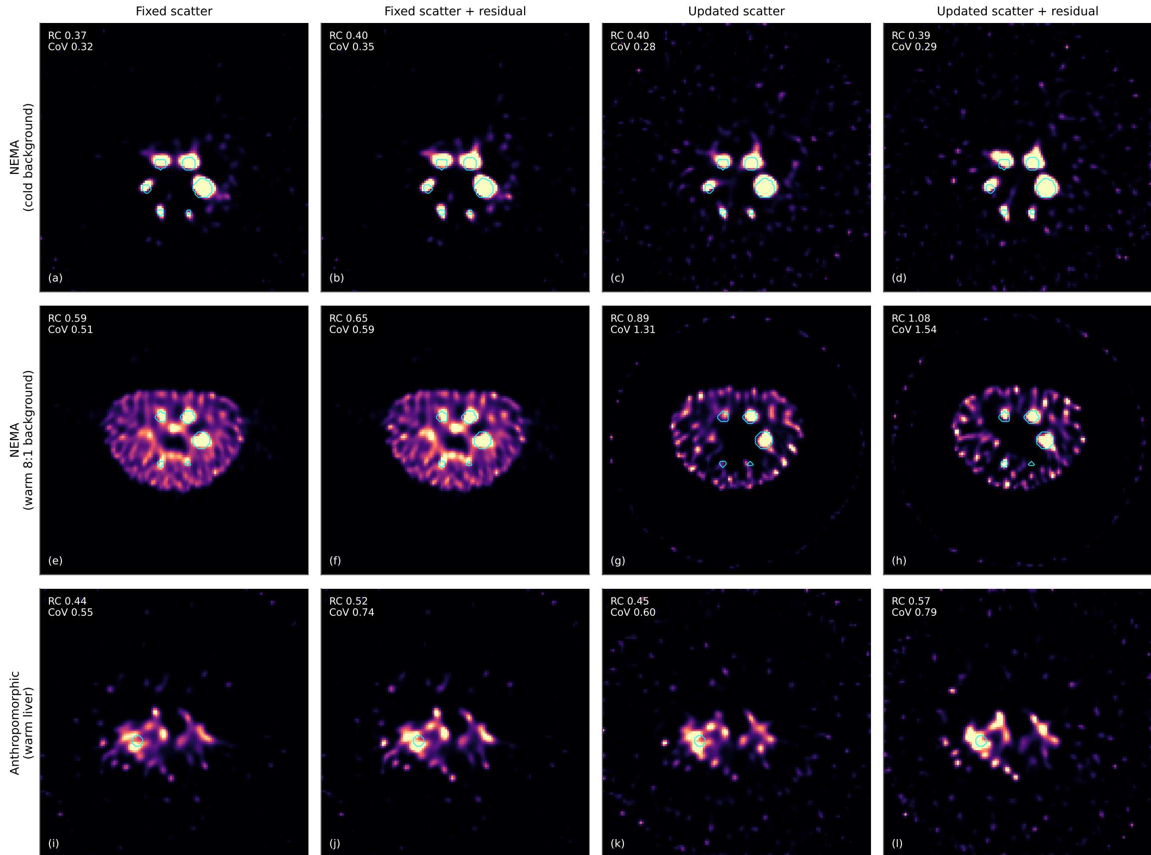
Reconstructed activity, four correction strategies ( \beta = 0.01 , range blur on, final iteration)
