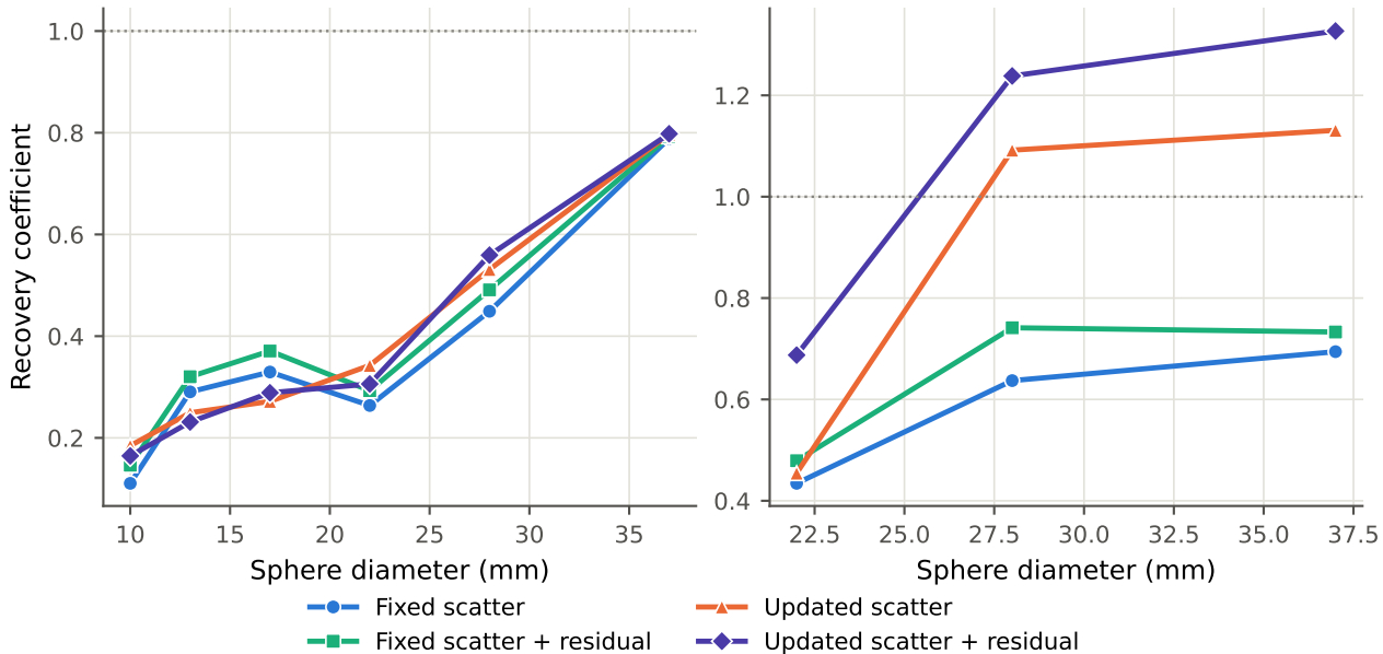
Resolution recovery vs sphere size ( \beta = 0.01 , brems blur on) NEMA (cold background) NEMA (warm 8:1 background)
