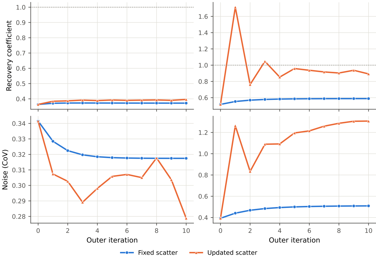
On-the-fly scatter update: convergence dynamics ( \beta = 0.01 ) NEMA (cold background) NEMA (warm 8:1 background)
