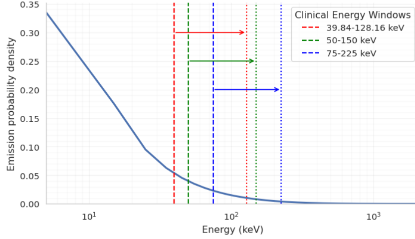
(a) Bremsstrahlung emission spectrum.
