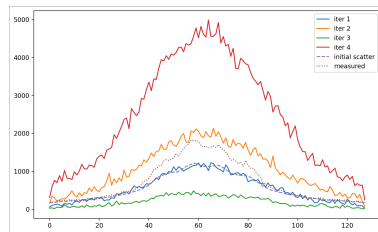
Figure 4.2: Figures showing profile through projections for NEMA phantom. Summed over projections, axial slice is through NEMA spheres. Horizontal axis show tangential coordinate on gamma camera, Vertical axis shows counts. Top, replacing additive data; bottom, damped addition of additive data ( \alpha = 0.2 ).
