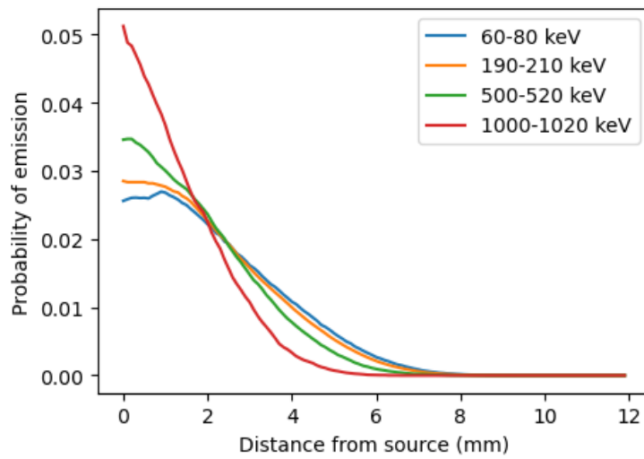
Figure 4.1: Plots showing probability of bremsstrahlung gamma emission versus the distance from ^{90}\text{Y} decay site. Data from Rault et al. [18]
