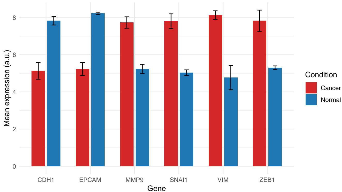
Mean gene expression (Normal vs Cancer)
