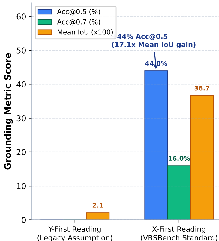
(b) Coordinate Order Ablation (150 Samples)
