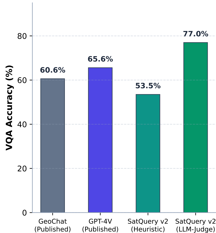
(a) VRSBench VQA Benchmark
