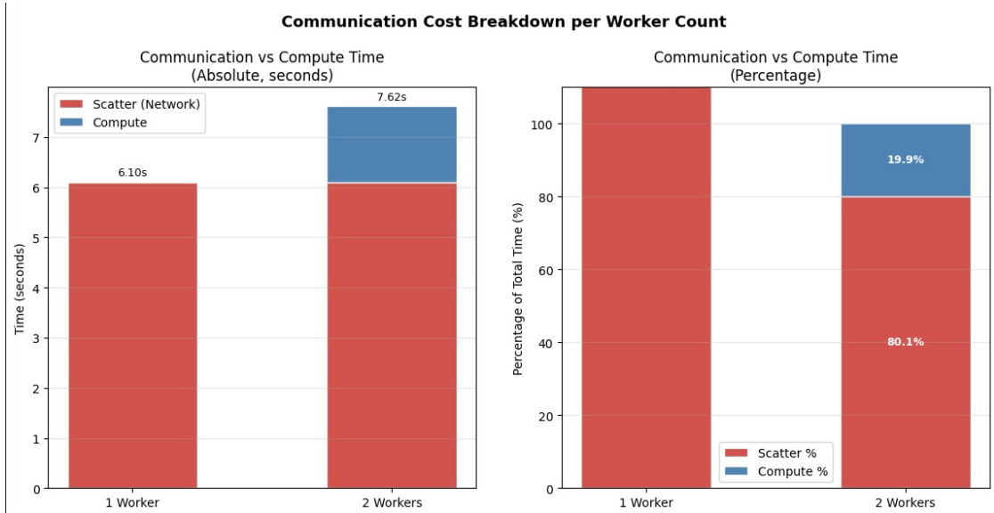
Figure 4: Communication vs Compute Time per Worker Count. Left panel shows absolute times in seconds (scatter cost in red, compute cost in blue). Right panel shows the percentage split. Scatter time (6.101 s) is constant because the test matrix is broadcast once regardless of worker count. The communication fraction decreases as worker count increases because compute work per worker decreases, but the fixed scatter overhead dominates for small label counts.
