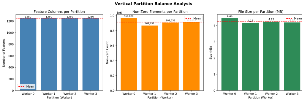
Figure 1: Partition Balance Analysis from Milestone 1. Each bar represents one of the 4 column shards. Feature counts and non-zero element densities are shown per partition to confirm that the vertical partitioning strategy distributed work evenly across workers.
