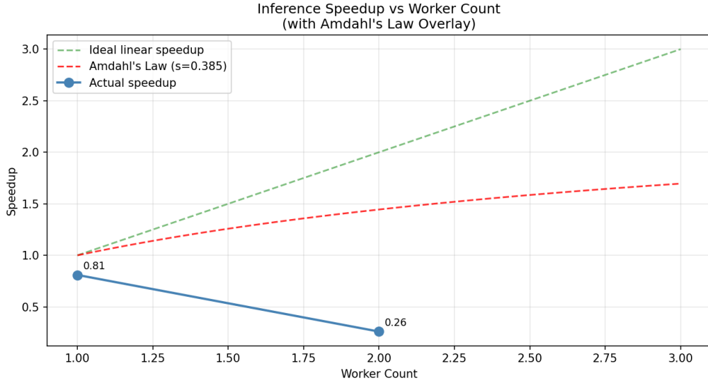
Figure 2: Inference Speedup vs Worker Count with Amdahl’s Law Overlay. The green dashed line represents ideal linear speedup; the red dashed line represents the Amdahl’s Law theoretical limit given the measured serial fraction ( s = 0.385 ); blue markers show actual measured speedup.
