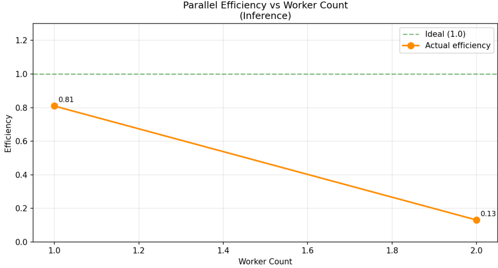
Figure 3: Parallel Efficiency vs Worker Count (Inference). Efficiency is defined as E = S/p where S is speedup and p is the number of workers. A value of 1.0 (green dashed) represents ideal efficiency. The drop from 1 to 2 workers is consistent with the high scatter-to-compute ratio in the 300-label benchmark.
