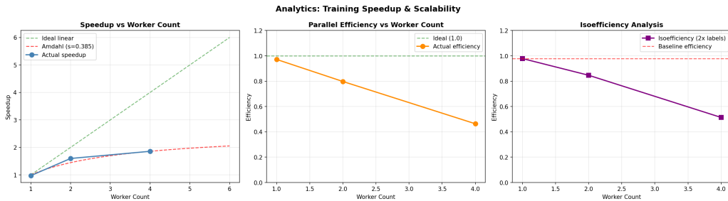
Figure 5: Milestone 2 Training Speedup and Efficiency vs Worker Count. The pattern mirrors the inference benchmarks: speedup improves with additional workers but falls below ideal linear scaling due to the communication overhead measured by the serial fraction of 38.5%.
