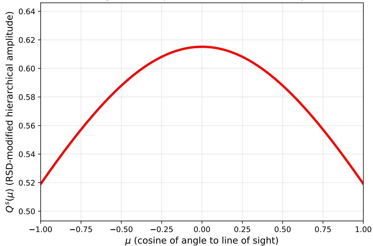
Configuration Dependence of Q in Redshift Space
