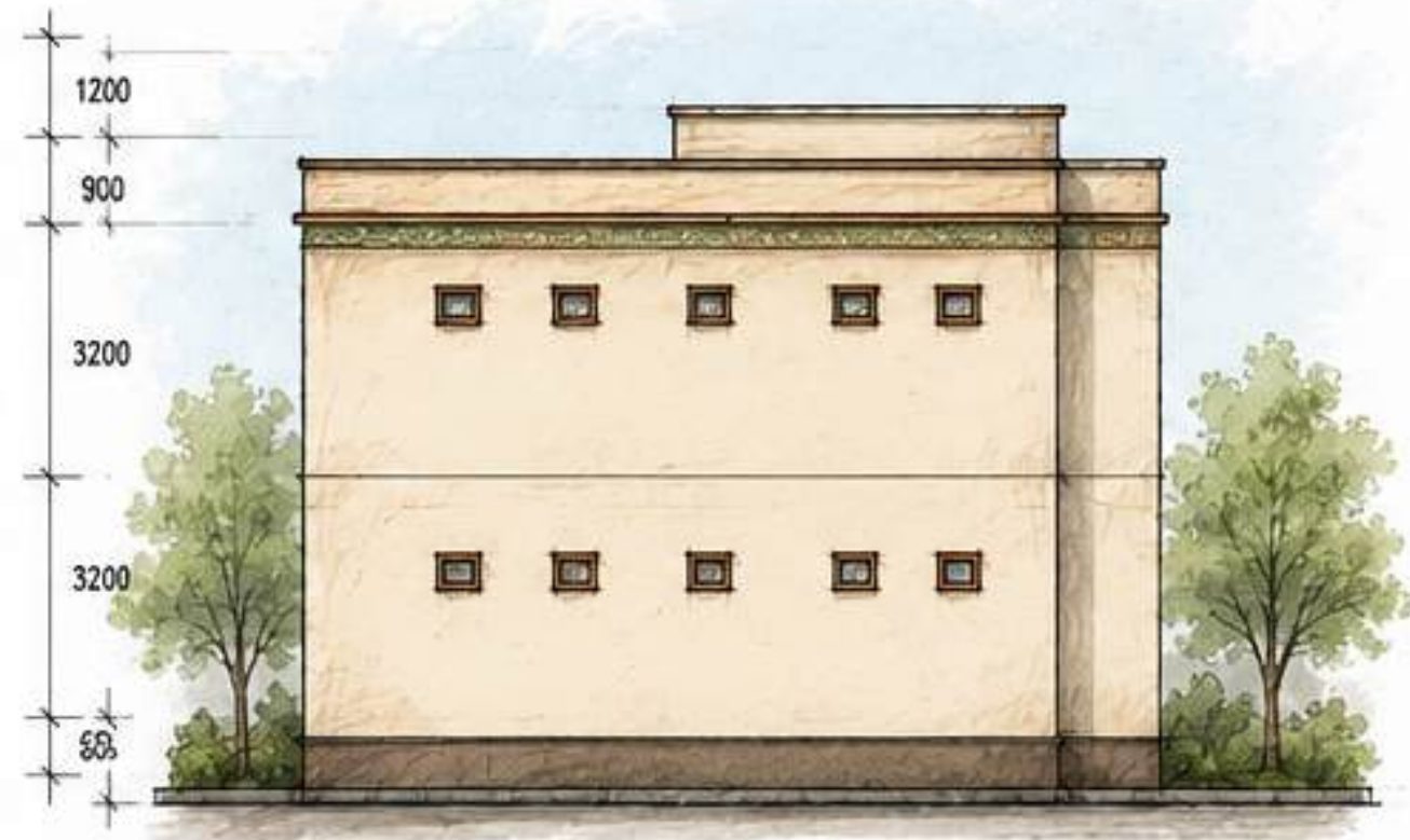
ELEVATION C
