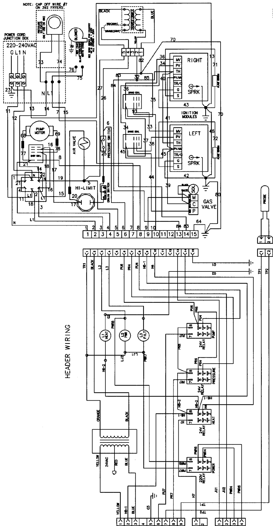
220-240 Volt FAST Wiring Diagram AP0803002 & below
