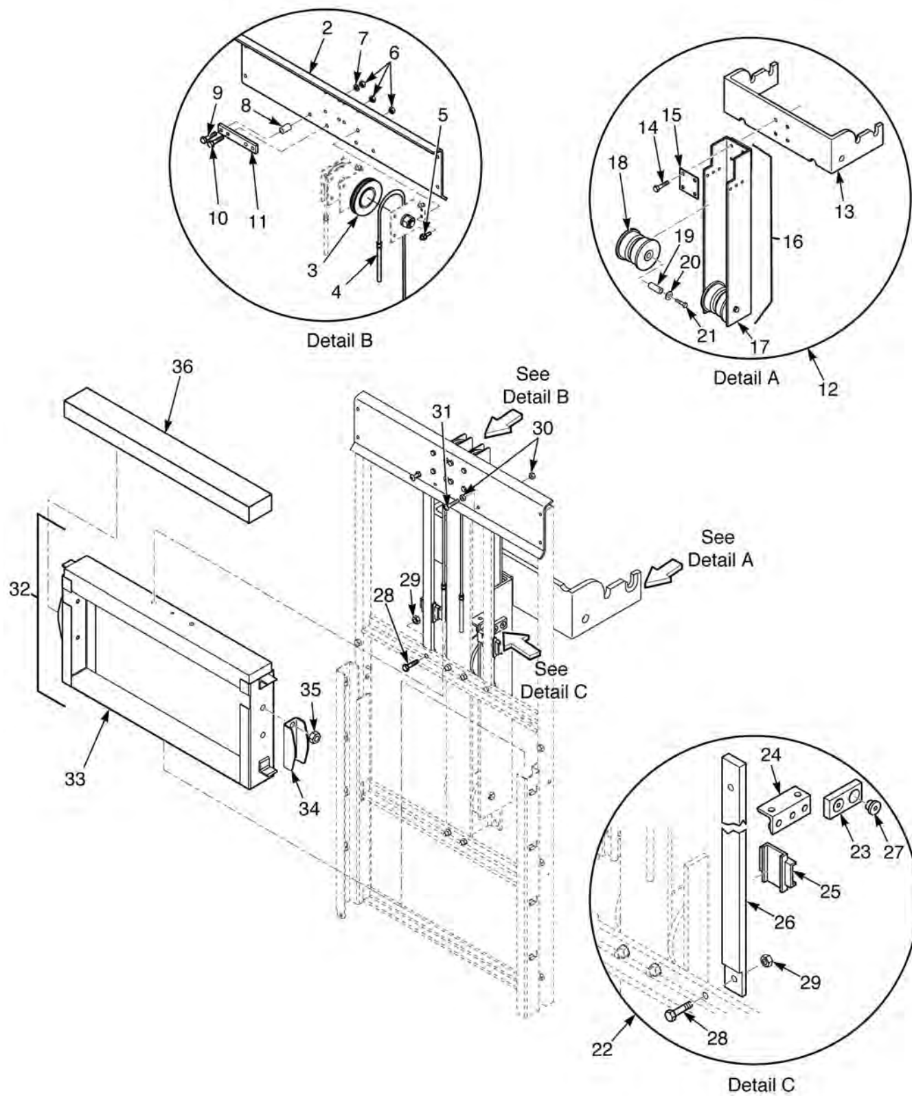
FIGURE 3-20. COUNTERWEIGHT & PULLEY SYSTEM (SN: AP0802028 & BELOW)
