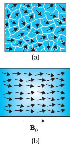
FIGURE 5.8 (a) Randomly oriented domains, (b) Aligned domains.
