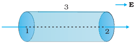
FIGURE 1.23 Calculation of the flux of uniform electric field through the surface of a cylinder.
