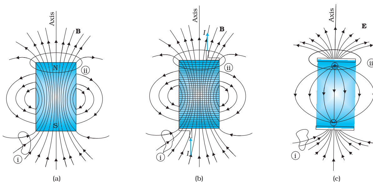
FIGURE 5.2 The field lines of (a) a bar magnet, (b) a current-carrying finite solenoid and (c) electric dipole. At large distances, the field lines are very similar. The curves labelled (i) and (ii) are closed Gaussian surfaces.
