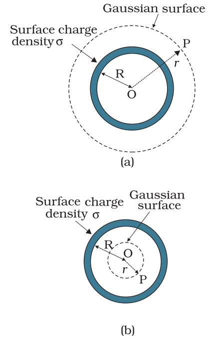
FIGURE 1.28 Gaussian surfaces for a point with (a) r > R , (b) r < R .
