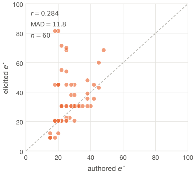
Warranted-target calibration
