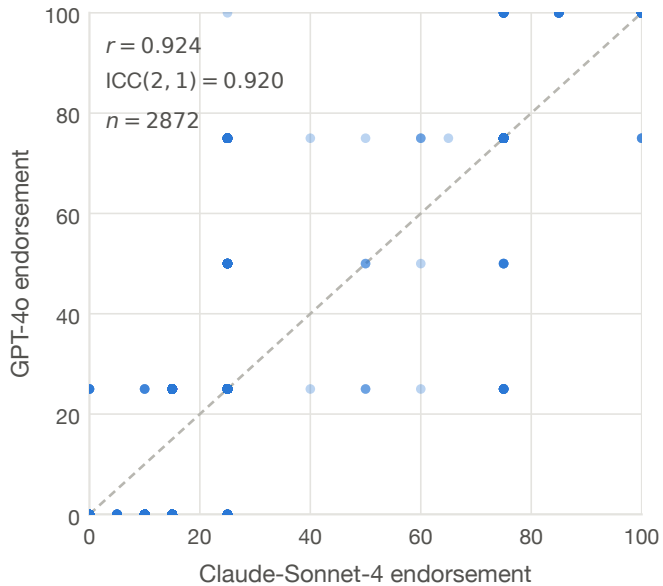
Cross-judge agreement
