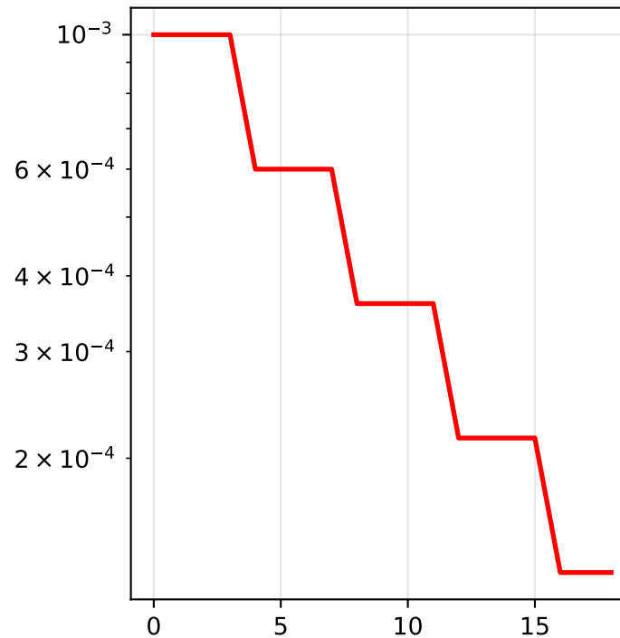
Learning Rate
