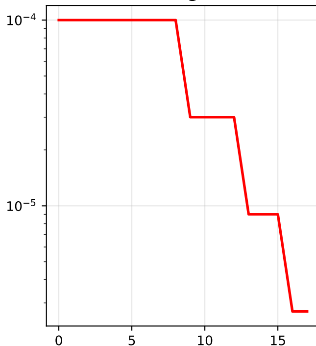
Learning Rate
