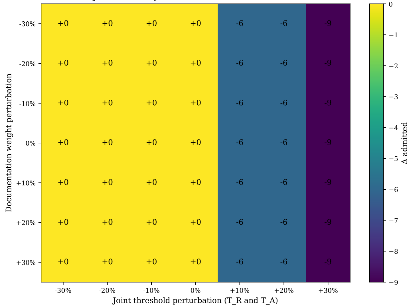
Joint sensitivity — Documentation — \Delta admitted
