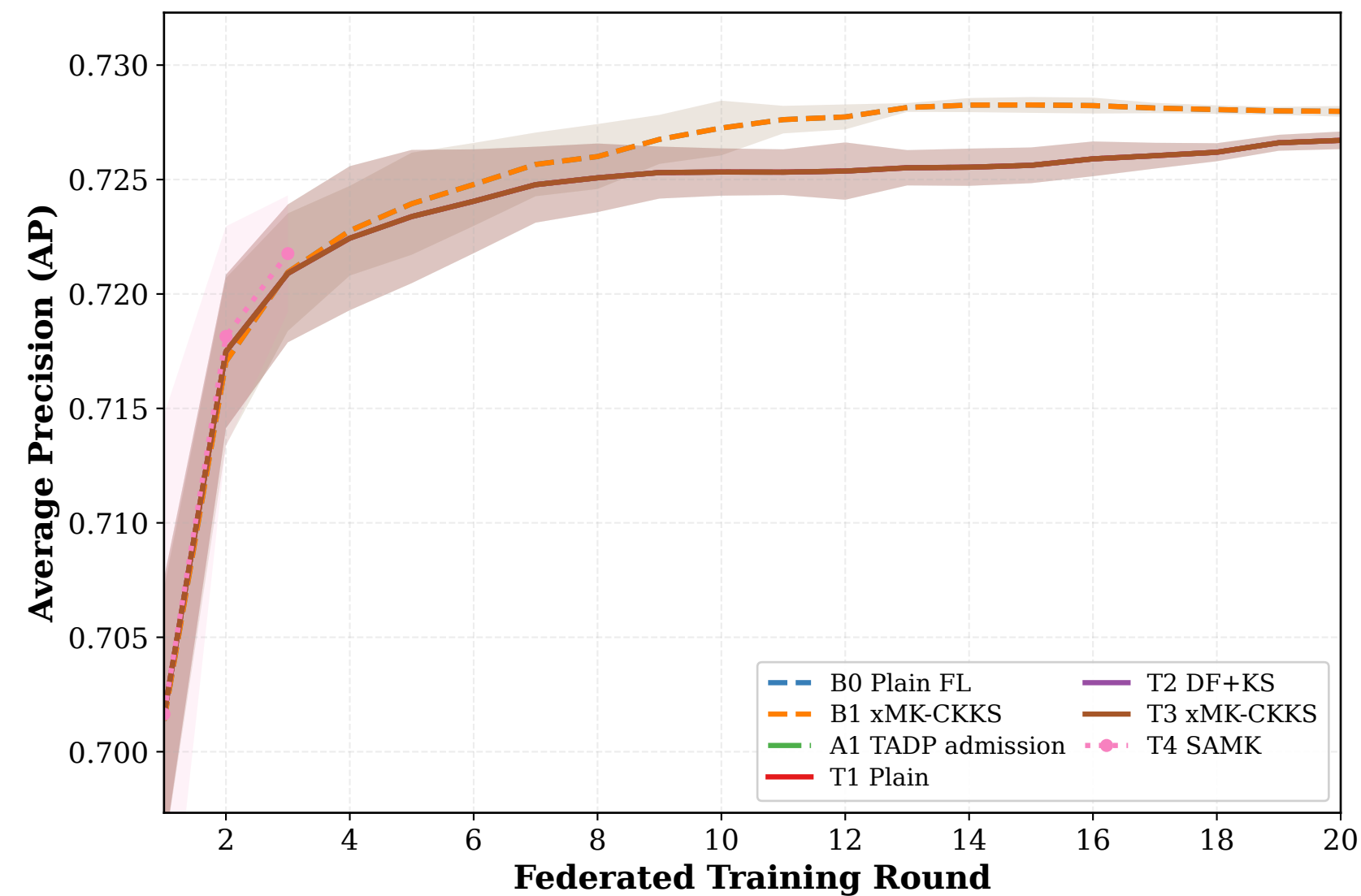
A) Average Precision (AP) Trajectories
