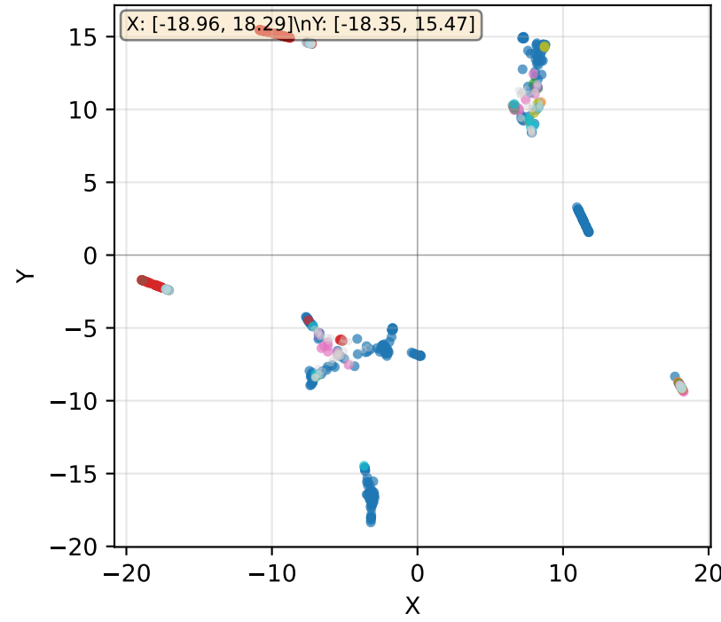
MDS - Raw
