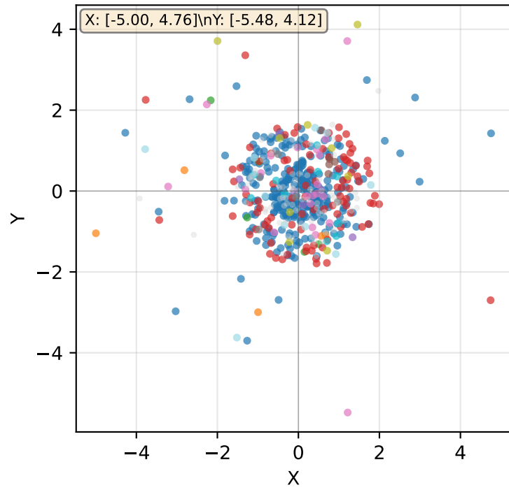
LocalMAP - Normalized
