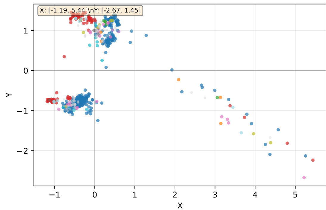
UMAP - Normalized
