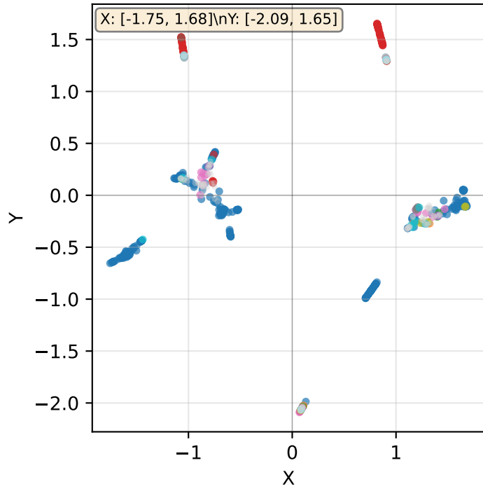
MDS - Normalized
