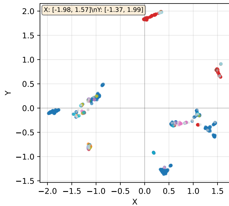
t-SNE - Normalized
