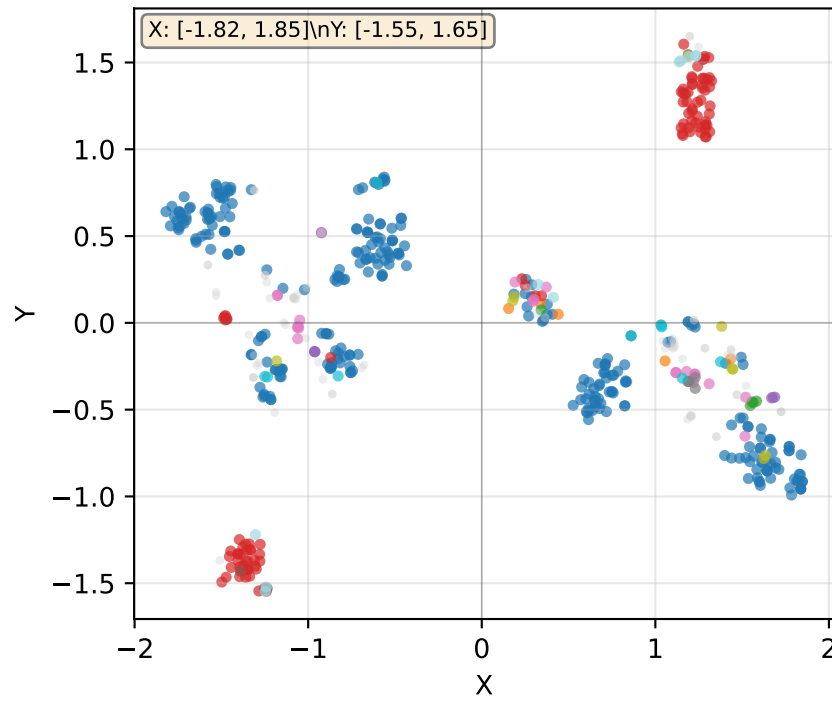
PaCMAP - Normalized
