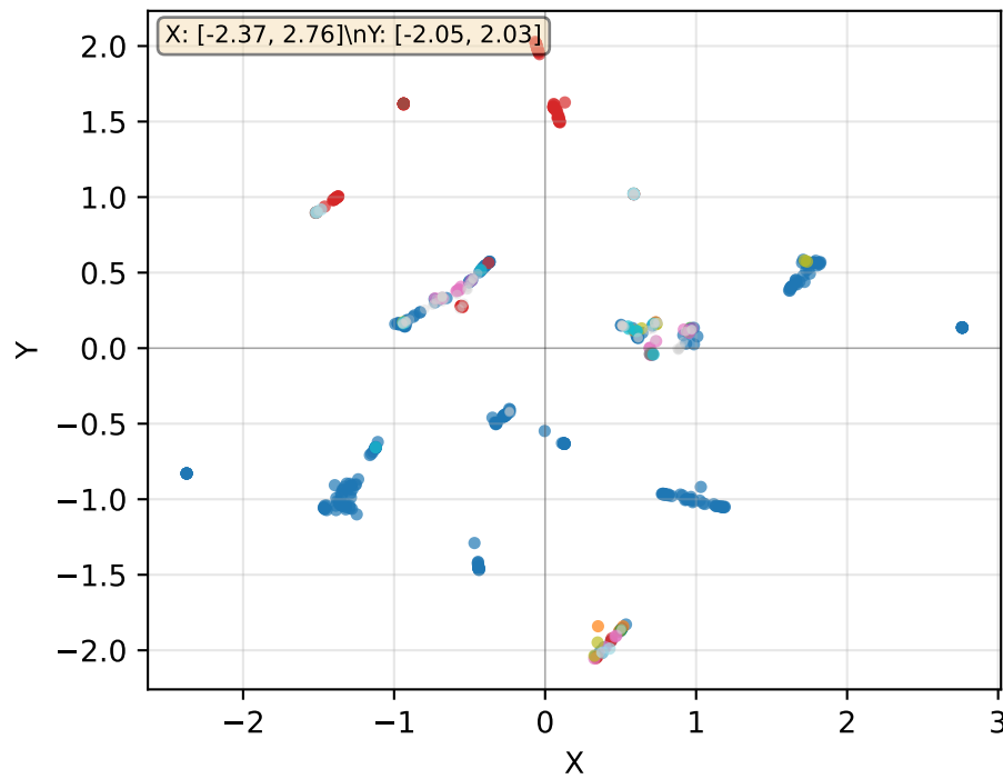
LocalMAP - Normalized
