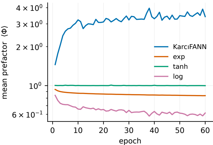
Step-size self-annealing — Dry Bean (7 classes)
