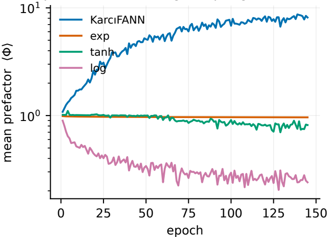
Step-size self-annealing — Optdigits (10 classes)
