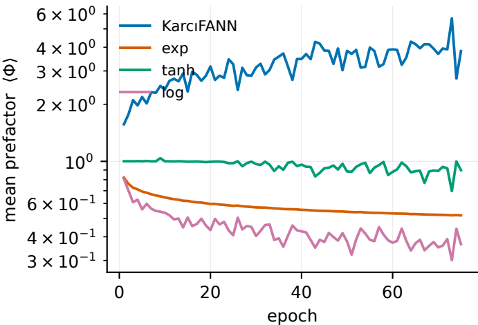
Step-size self-annealing — Pendigits (10 classes)
