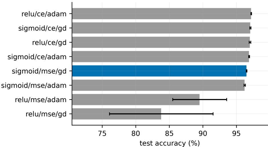
Configuration ablation — MNIST (10 classes)
